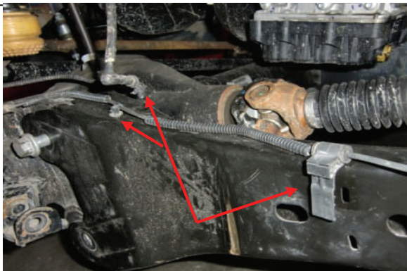
Remove all wiring clips from radius arms
