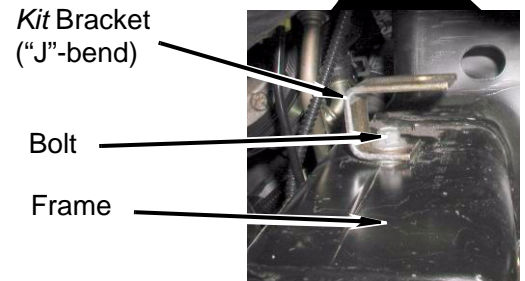
Install kit washers (7/16") between the kit brackets and the frame
