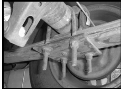
Picture shown with DJM spring plate.
