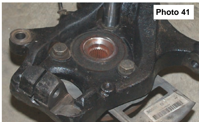
Photo 41 Remove Wheel Bearing Assembly from Stock Knuckle
