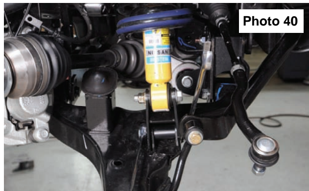
Photo 40 Install Strut Assembly On Lower Control Arm
