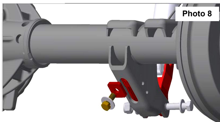
Install Magneride shock relocation brackets.
