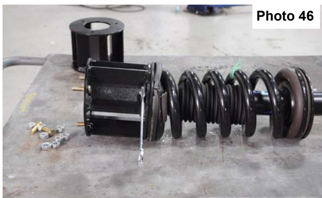
Install strut spacer with the shorter side toward the frame.
