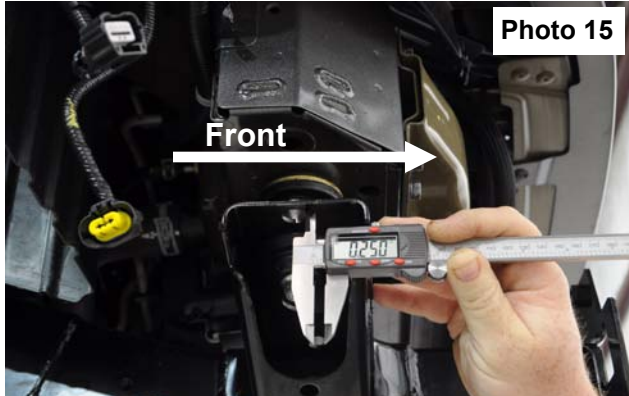
Measure 1/4" to the front of truck and mark.
