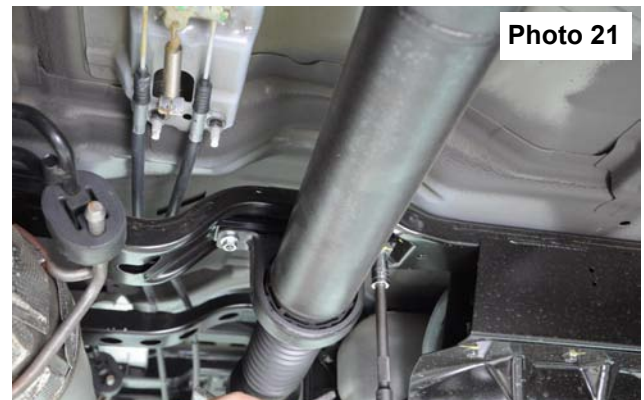
Tighten carrier bearing bracket.
