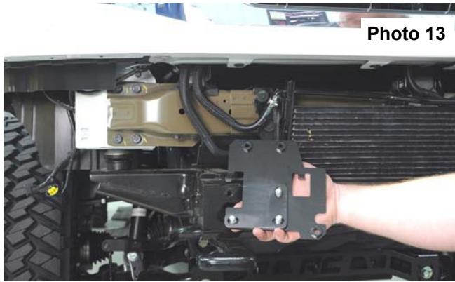
Install bumper shims and hardware.
