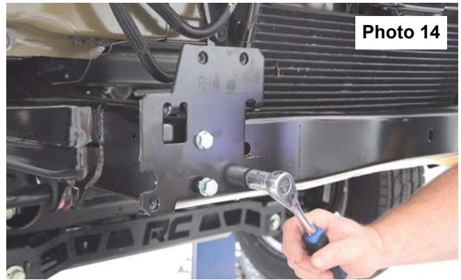
Install mounting plates on frame.
