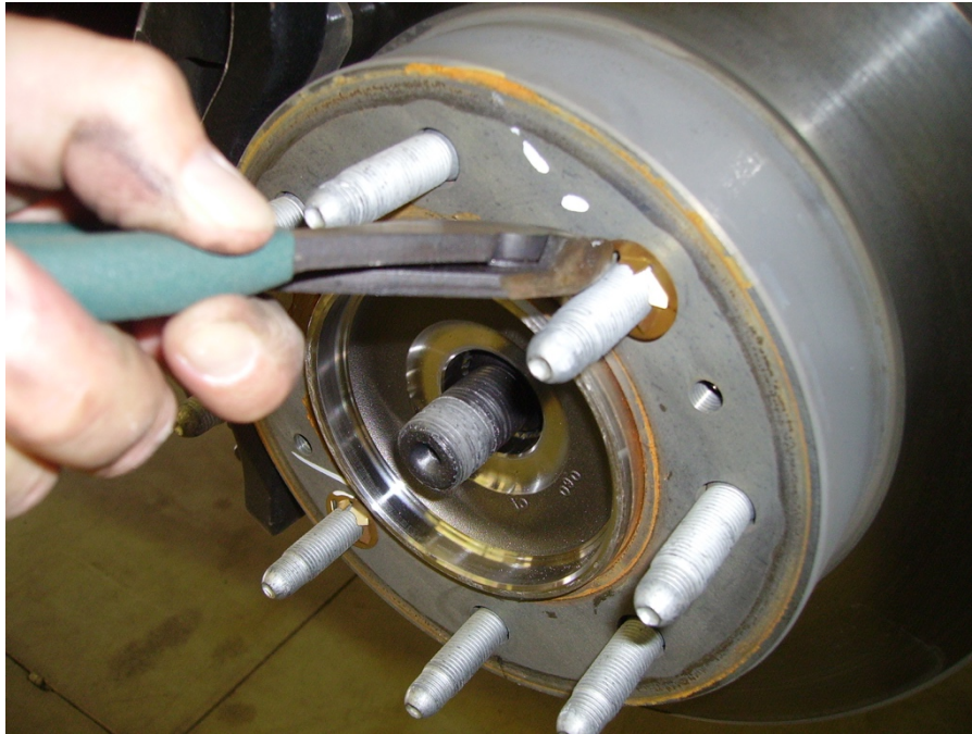
Figure 3 Remove clips from all 4 corners of vehicle. MUST DO for aftermarket wheels.
