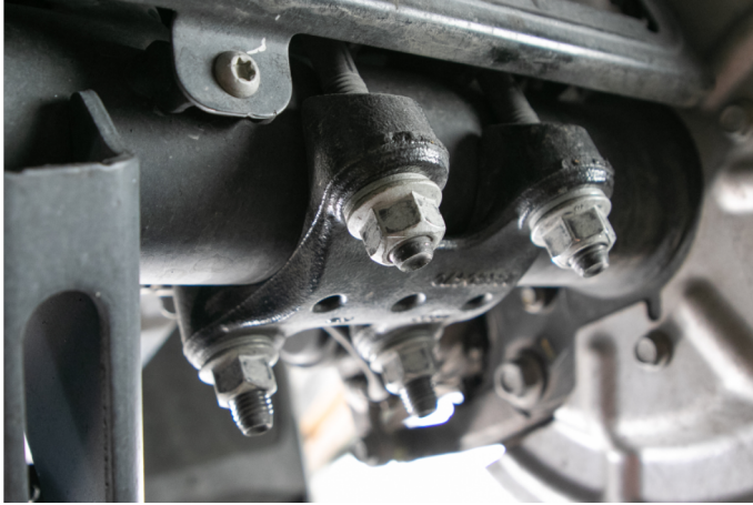
Figure 2: Remove Factory U-bolts
