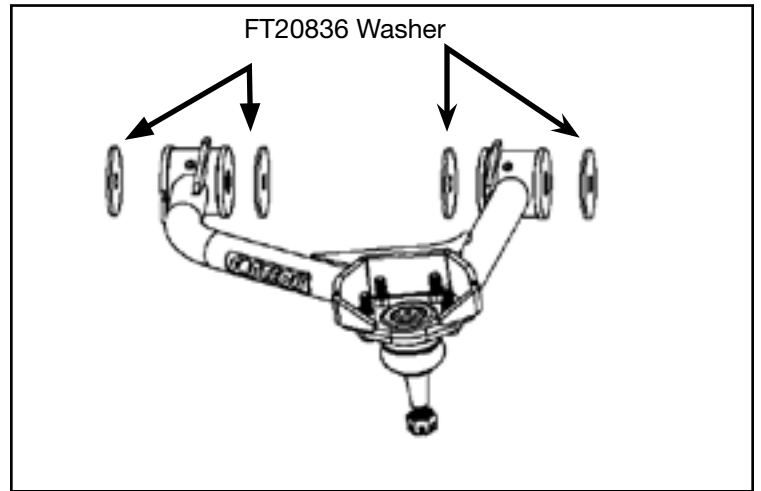
FIGURE 35 - STEP 26
