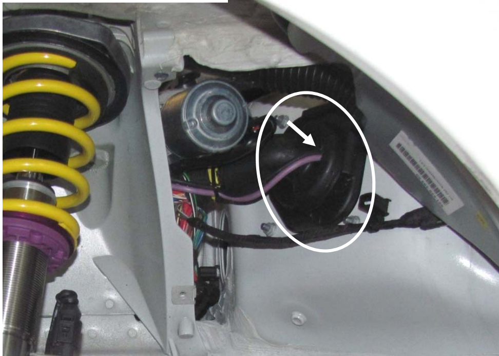
Montageposition 11 / Assembly position 11
