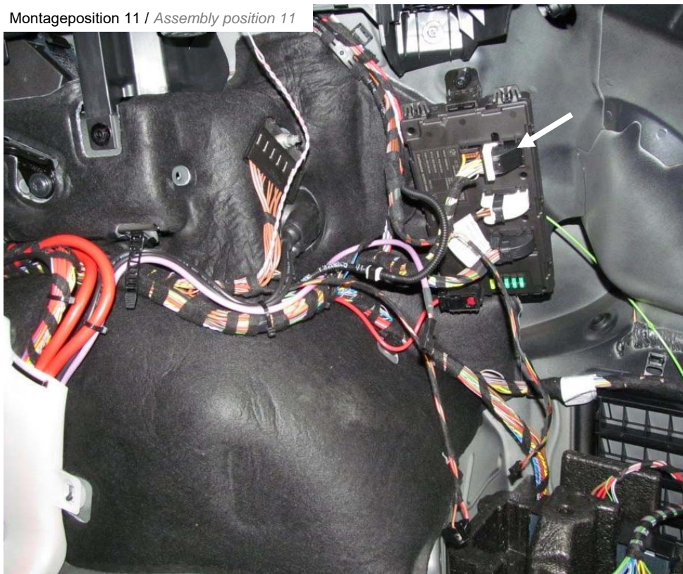
Montageposition 11 / Assembly position 11
