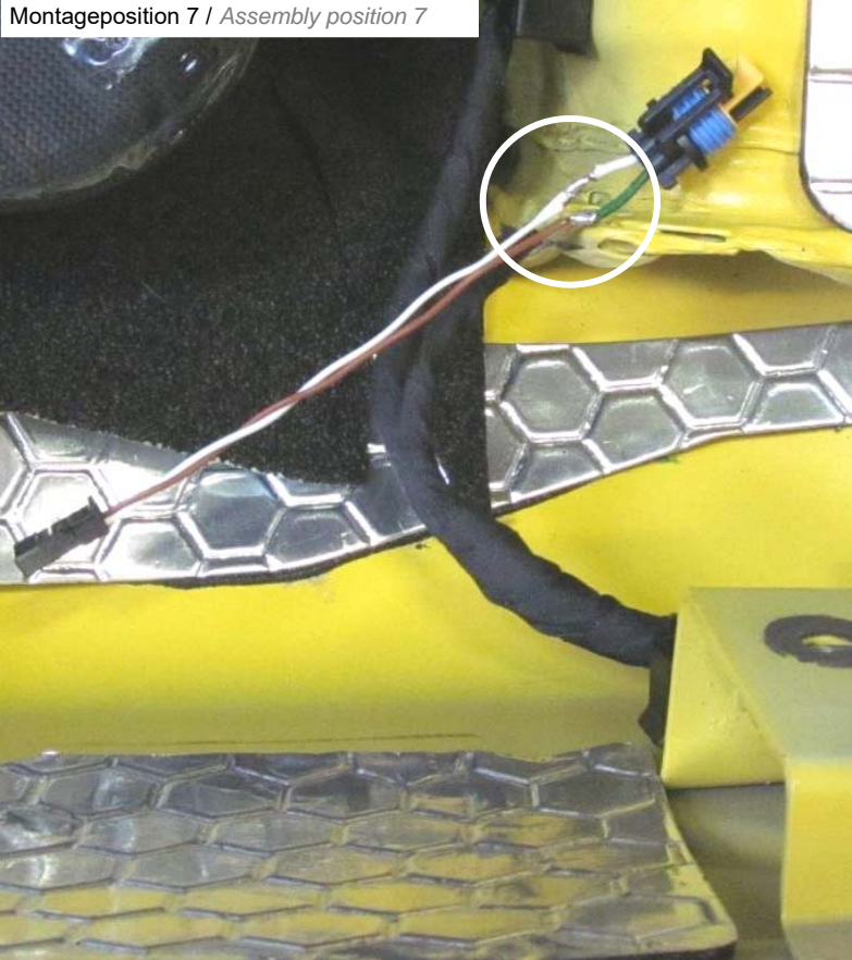
Montageposition 7 / Assembly position 7
