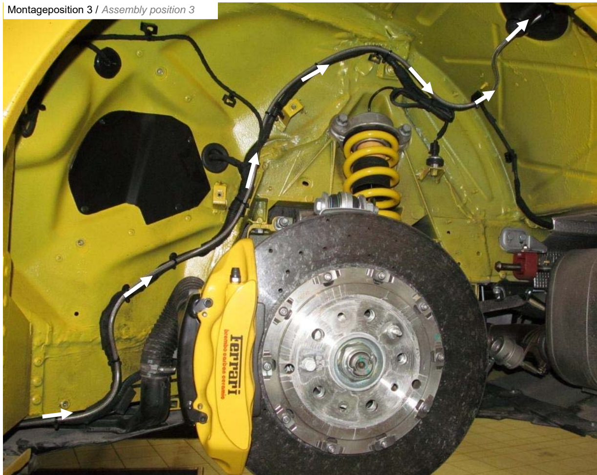
Montageposition 3 / Assembly position 3
