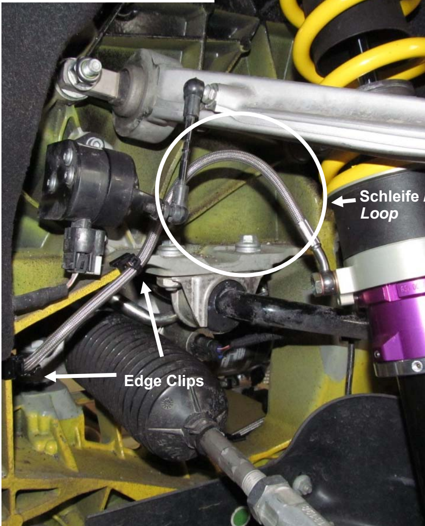
Montageposition 1 / Assembly position 1
