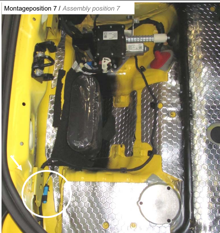
Montageposition 7 / Assembly position 7
