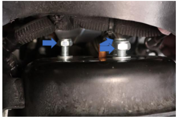
Step 17. Install the 3 17mm bolts provided with the kit along with washers on top of the shock tower. Torque nuts to 52 Ft. Lbs.
