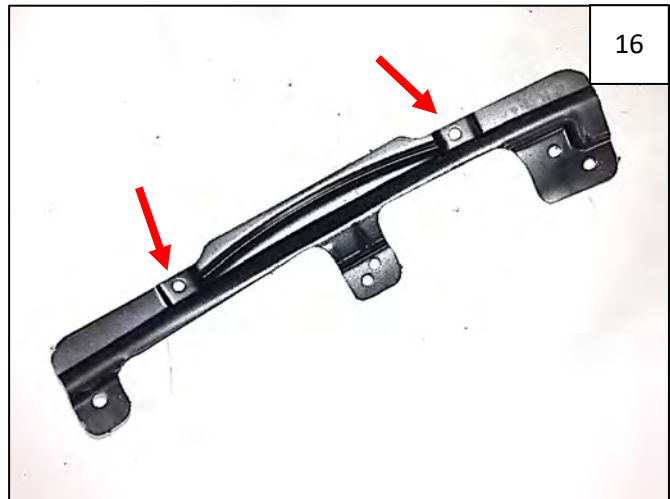
Front Inner Bracket Short "U" Clip locations.
