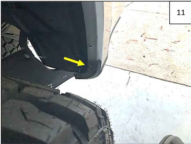
Remove factory fastener on rear splash shield.
