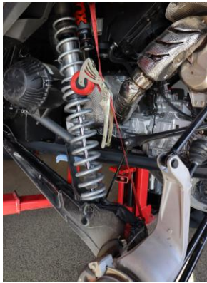
Step 27. Remove strap securing trailing arm to frame.
