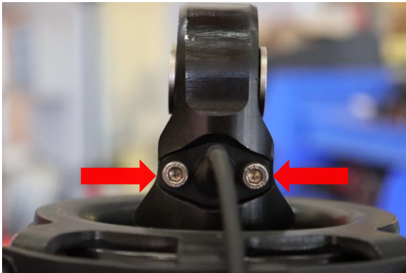
Step 21. Install lower shock wire harness using both 4mm allen head screws. Tighten to manufacturer specification.
