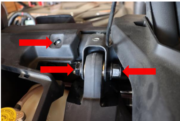
Step 23. Install upper shock mount nut and bolt. Tighten to manufacturer specification using 21mm wrench and socket. Install T30 bolt from step 6 and tighten to manufacturer specification.
