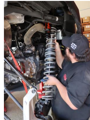
Step 22. Set shock assembly in vehicle by inserting top of assembly through opening in body panels and setting lower shock mount in trailing arm.
