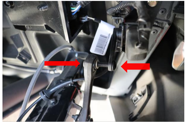
Step 28. Install ride height sensor arm at front of lower trailing arm using T30 bolt and 10mm nut. Tighten to manufacturer specification.
