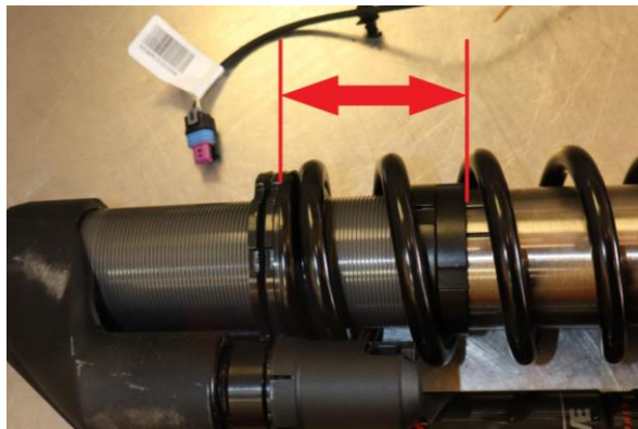
Step 17. Set crossover ring to 70mm (2 3/4in.) from bottom of spring seat to bottom of crossover ring.
