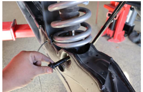
Step 24. Install lower shock mount nut and bolt. Tighten to manufacturer specification using 2 21mm sockets.
