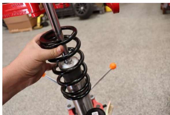
Step 15. Remove OE secondary spring.
