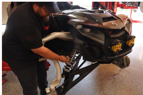
Step 23. Install shock in vehicle using upper mount bolt to hold assembly in place.
