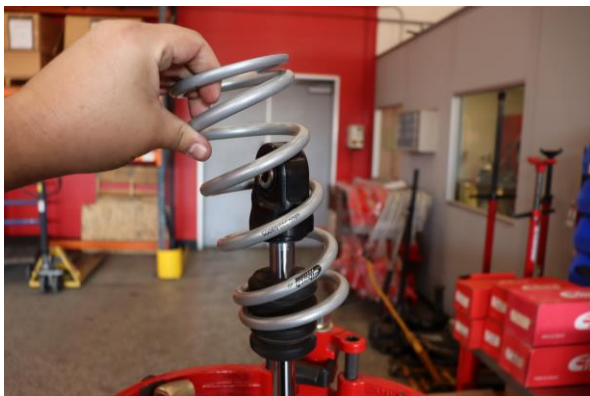
Step 18. Install Eibach secondary spring.
