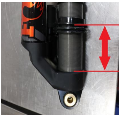
Step 16. Set pre-load spring seat to 75mm (2 15/16in.) from bottom of seat to bottom of reservoir bridge.
