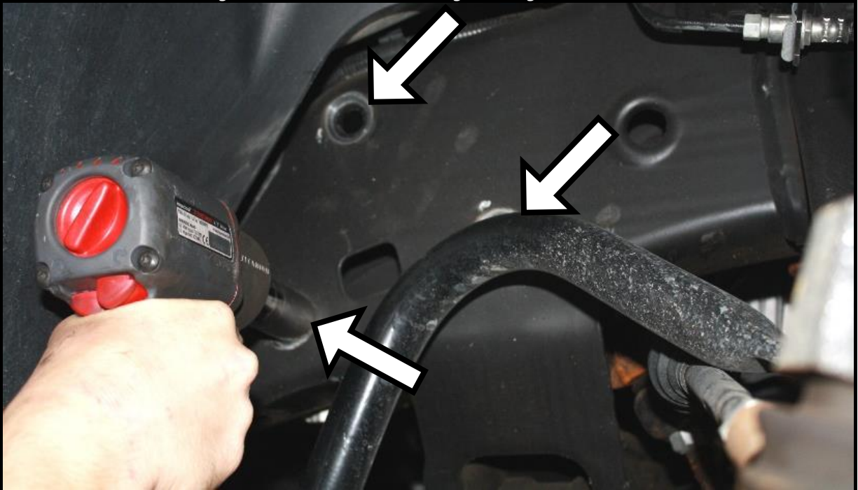
Figure 5: Remove Bolts Holding Steering Box to Frame
