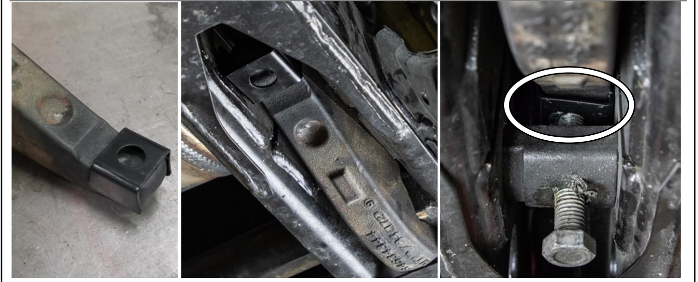
Figure 75: Cognito Torsion Key Retainer
