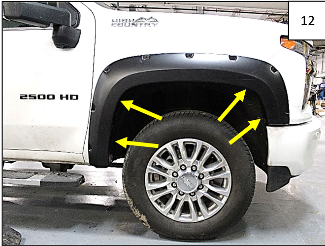
Reinstall 4 factory screws through holes in flare and into holes in fender.
