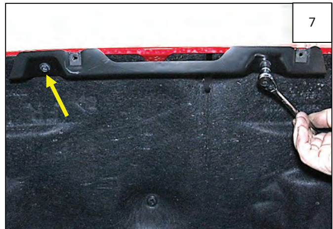
Align holes in Inner Bracket with uppermost holes in fender. Start 2 supplied 20mm Hex Screws through Inner Bracket and into holes in fender. Tighten screws.
