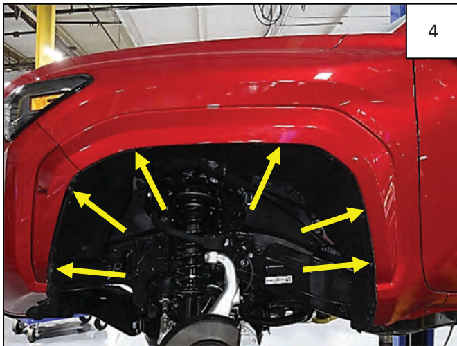
Remove 6 factory screws from wheel well as indicated by arrows.
