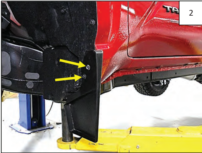
If factory mudflap is present, remove 2 factory screws indicated by arrows.
