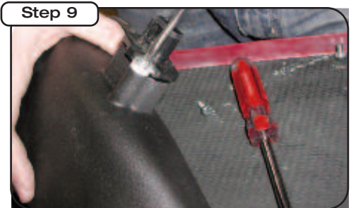
Step 9 Transfer the MAF sensor from the factory airbox to the new intake tube. Make sure you use the provided spacers and gasket between sensor and tube. Install the threaded hose fitting onto the tube.
