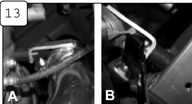
13 A)Position upper tab to M8 isolation mount. B)Now from on top of vehicle secure tab using M8 nut and washer and tighten using 13mm wrench.
