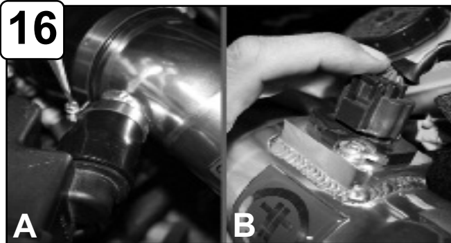
16 A) Attach 05-01043 coupling from the crank case port on the intake, to the stock plastic vacuum port. B) Re-connect MAF sensor harness.
